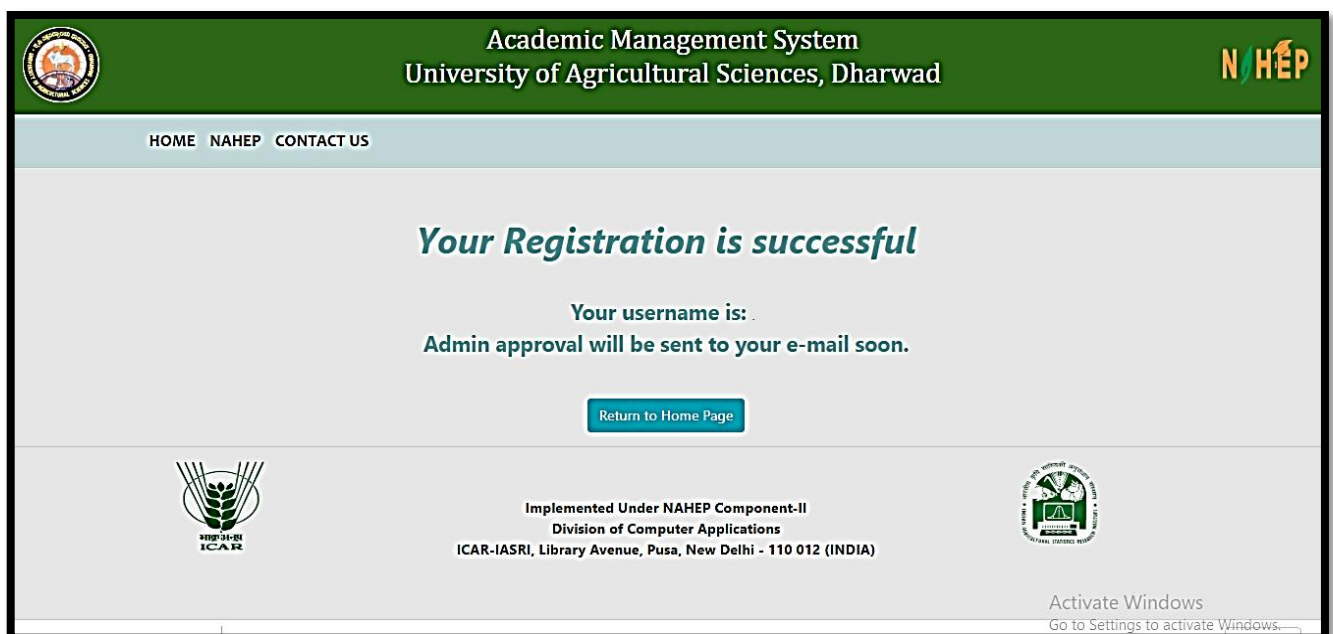
Fig. 2.2 Registration Successfully
